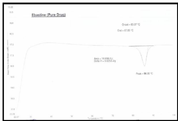
Figure 2: DSC thermogram of pure Ebastine
