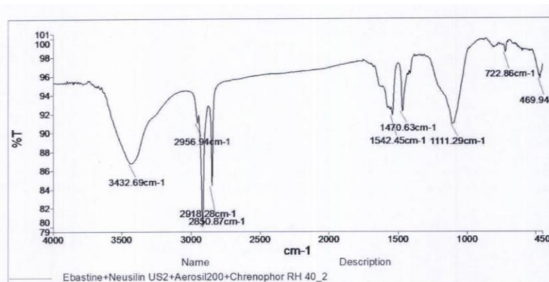
Figure 5: Drug-excipient compatibility FTIR spectra
