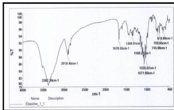
Figure 1: FTIR spectrum of pure Ebastine
